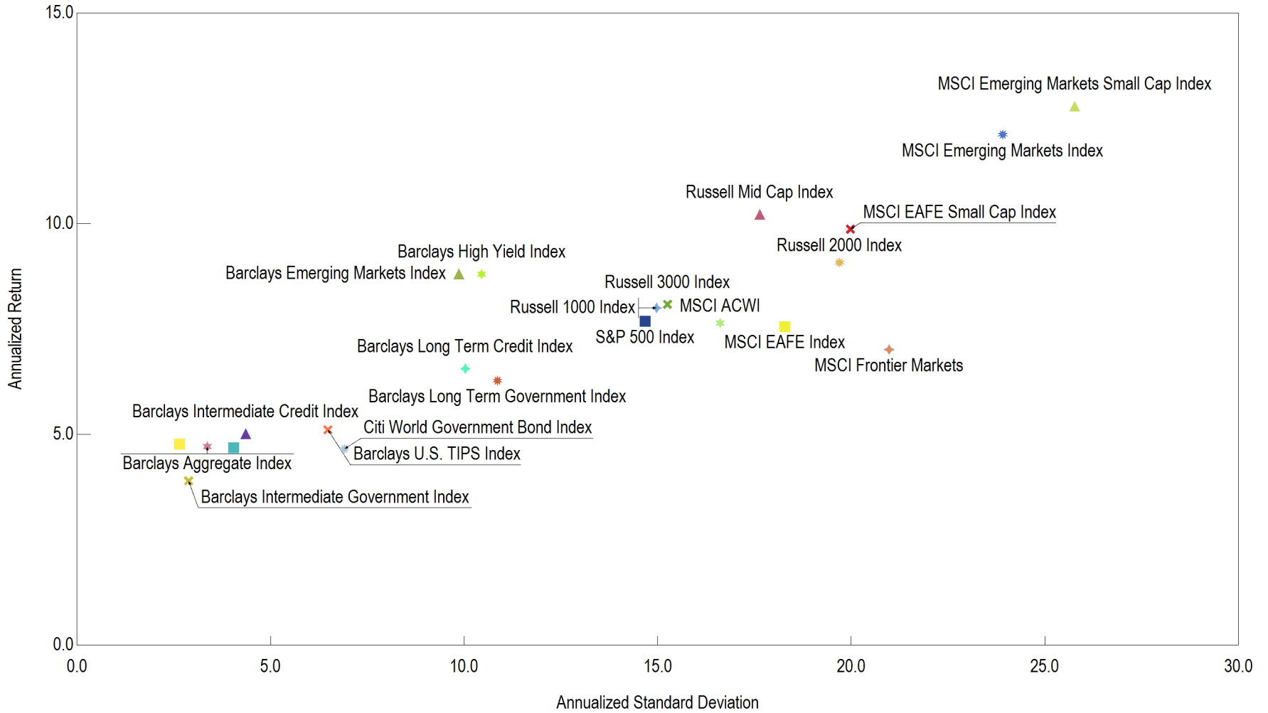
Annualized Return vs. Annualized Standard Deviation 10 Years Ending November 30, 2013
