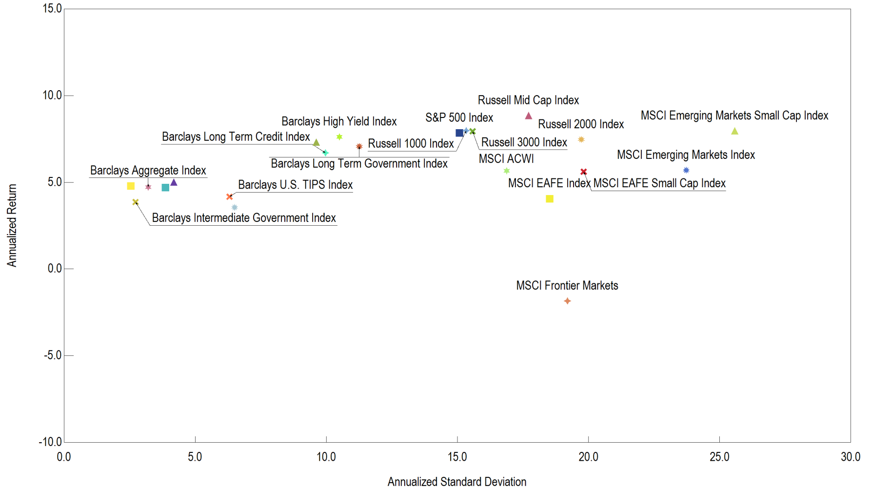
Annualized Return vs. Annualized Standard Deviation 10 Years Ending October 31, 2015
