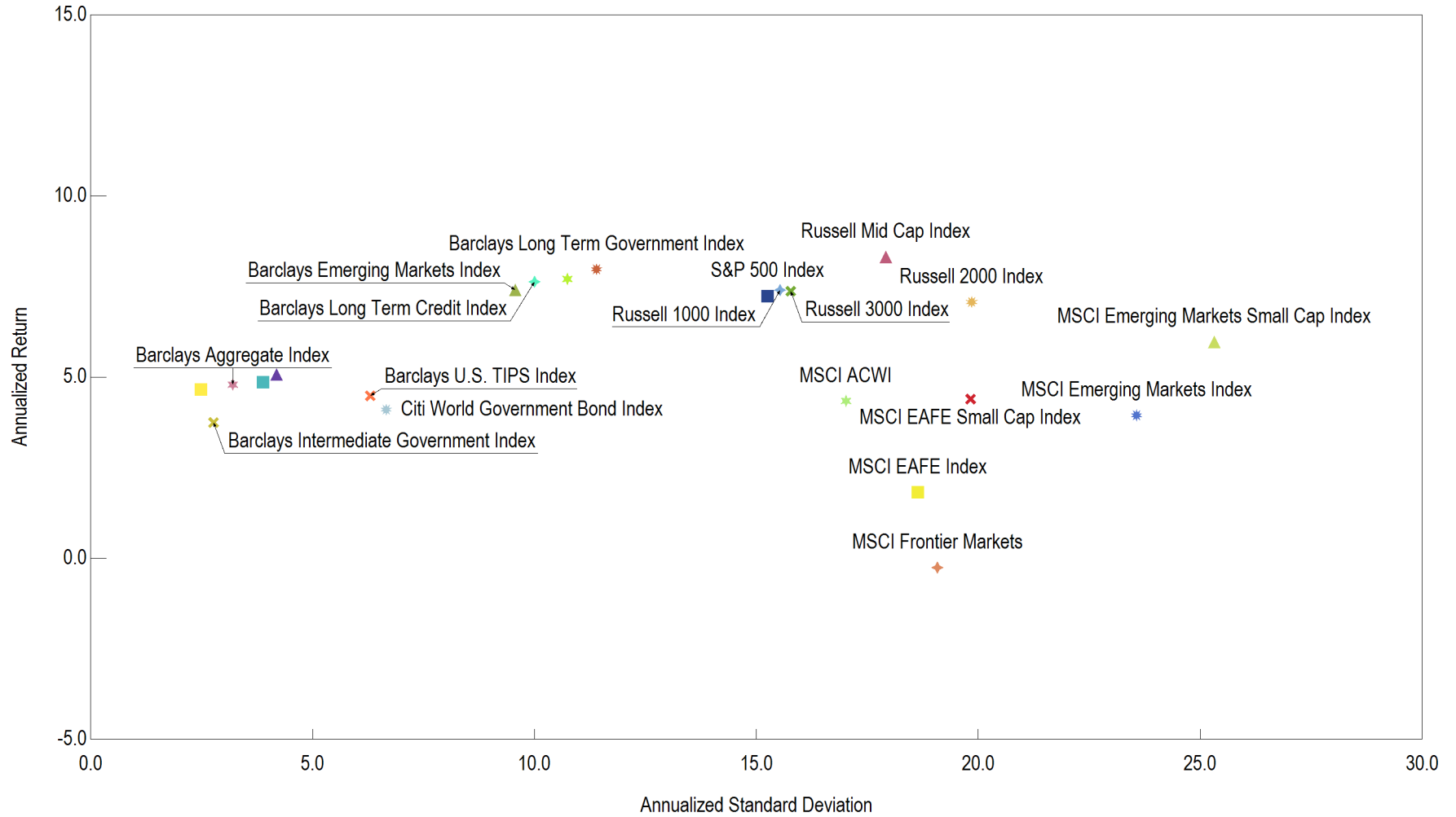
Annualized Return vs. Annualized Standard Deviation 10 Years Ending September 30, 2016
