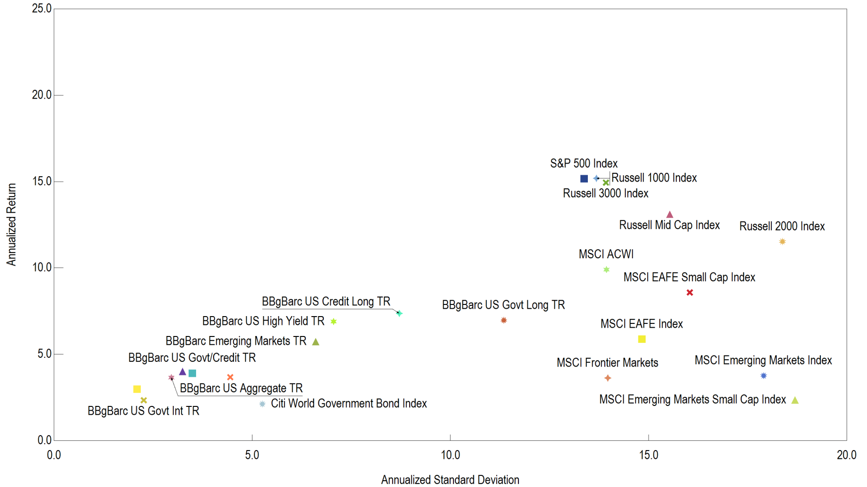
Annualized Return vs. Annualized Standard Deviation 10 Years Ending August 31, 2020
